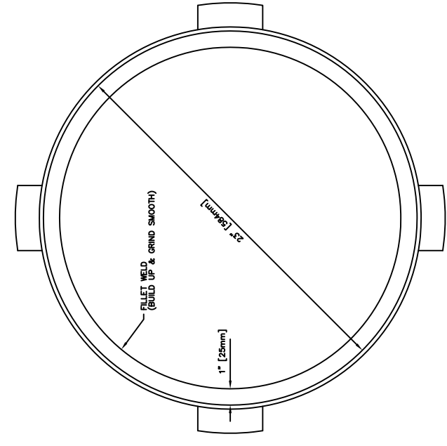
BOTTOM VIEW SCALE 3/8" = 1'-0"
